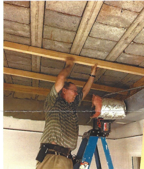
Co-worker Chuck Saunders placing joists to hold sound barrier and dense insulation for new ceiling
